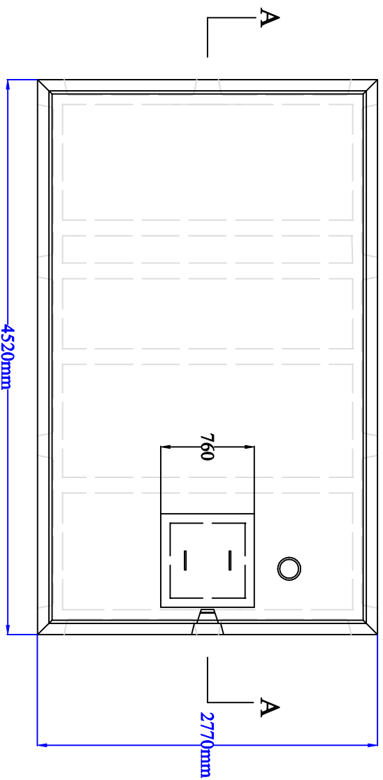
TOP VIEW
